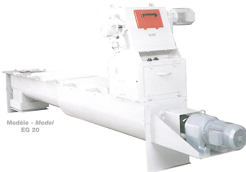
Vis d'enrobage. Coating screw conveyor.
